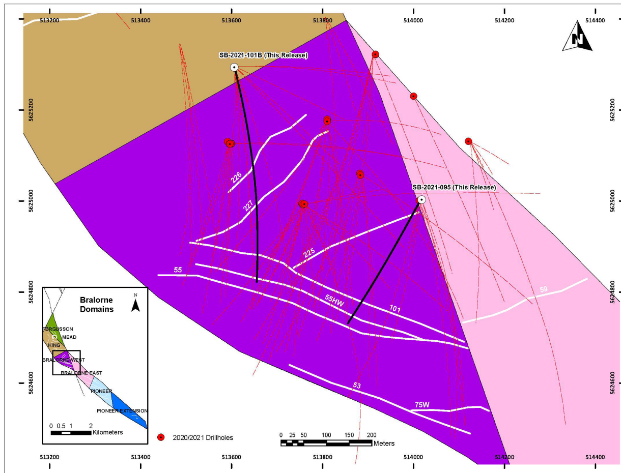
Figure 3: SB-2021-095 and 101B drill hole locations with the Bralorne West block.
