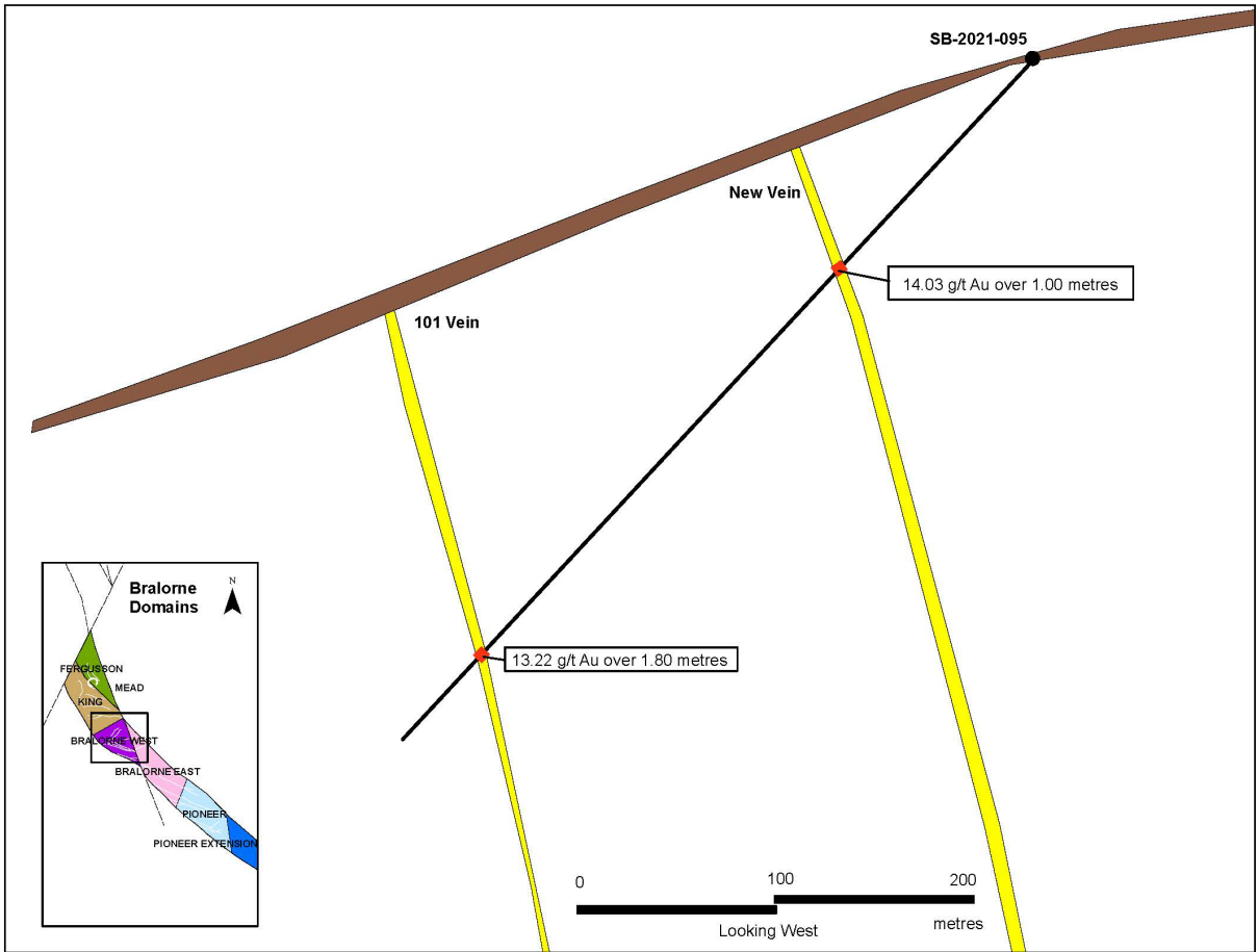
Figure 1: SB-2021-095 cross section with vein intersections and grade.
