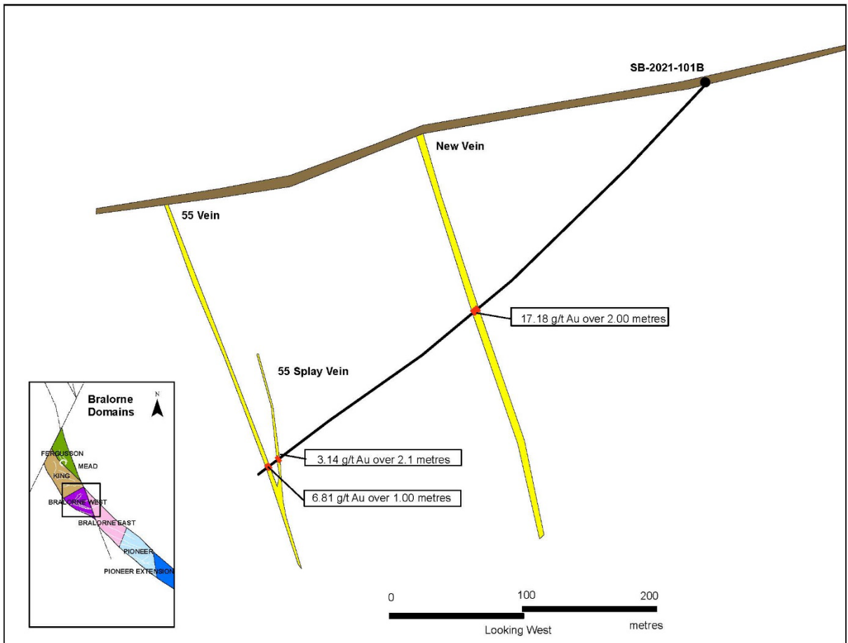
Figure 2: SB-2021-101B cross section with vein intersections and grade.
